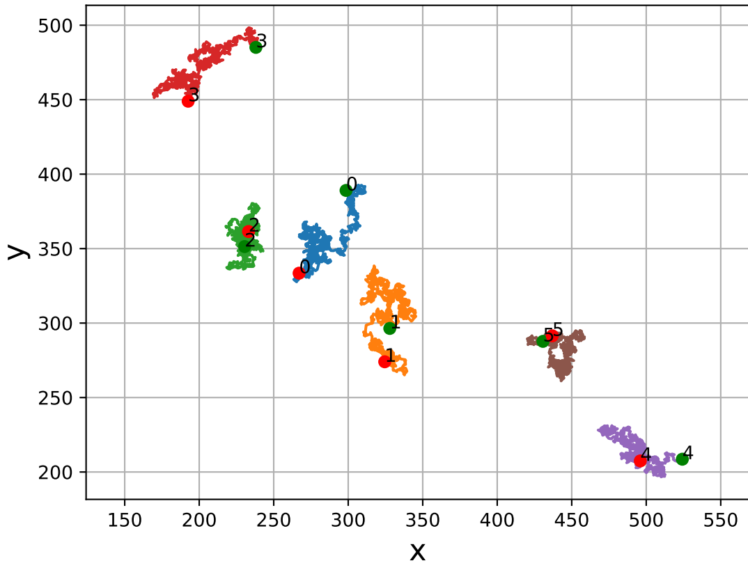
2D Brownian Motion with mirror boundary conditions.
