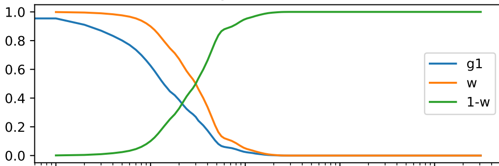
Correlation data @ k = (12,2)
