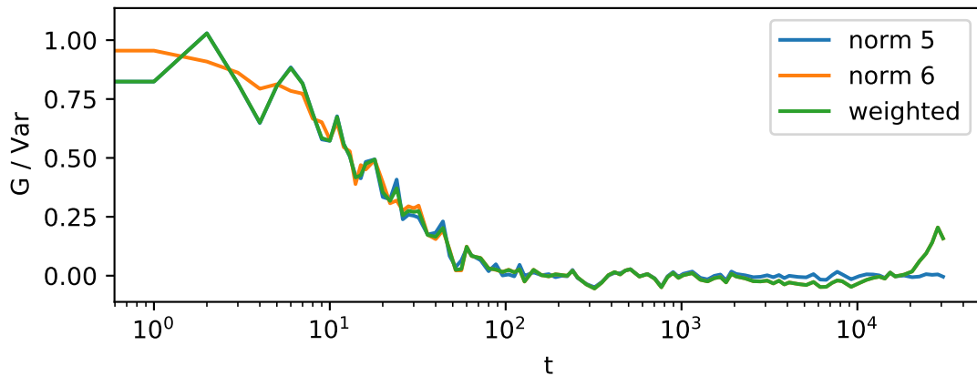
Correlation data @ k = (12,2)
