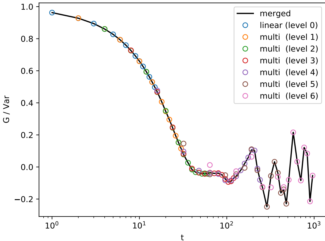
Multilevel data @ k = (4,12)
