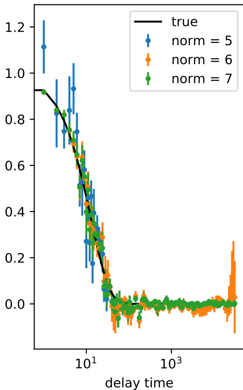
Correlation @ k =(16,0)
