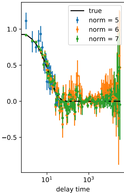
Correlation @ k =(16,0)
